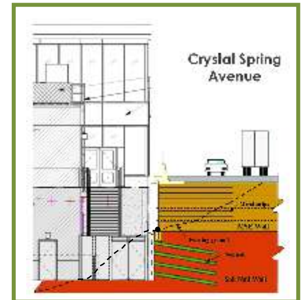
RETAINING WALL
